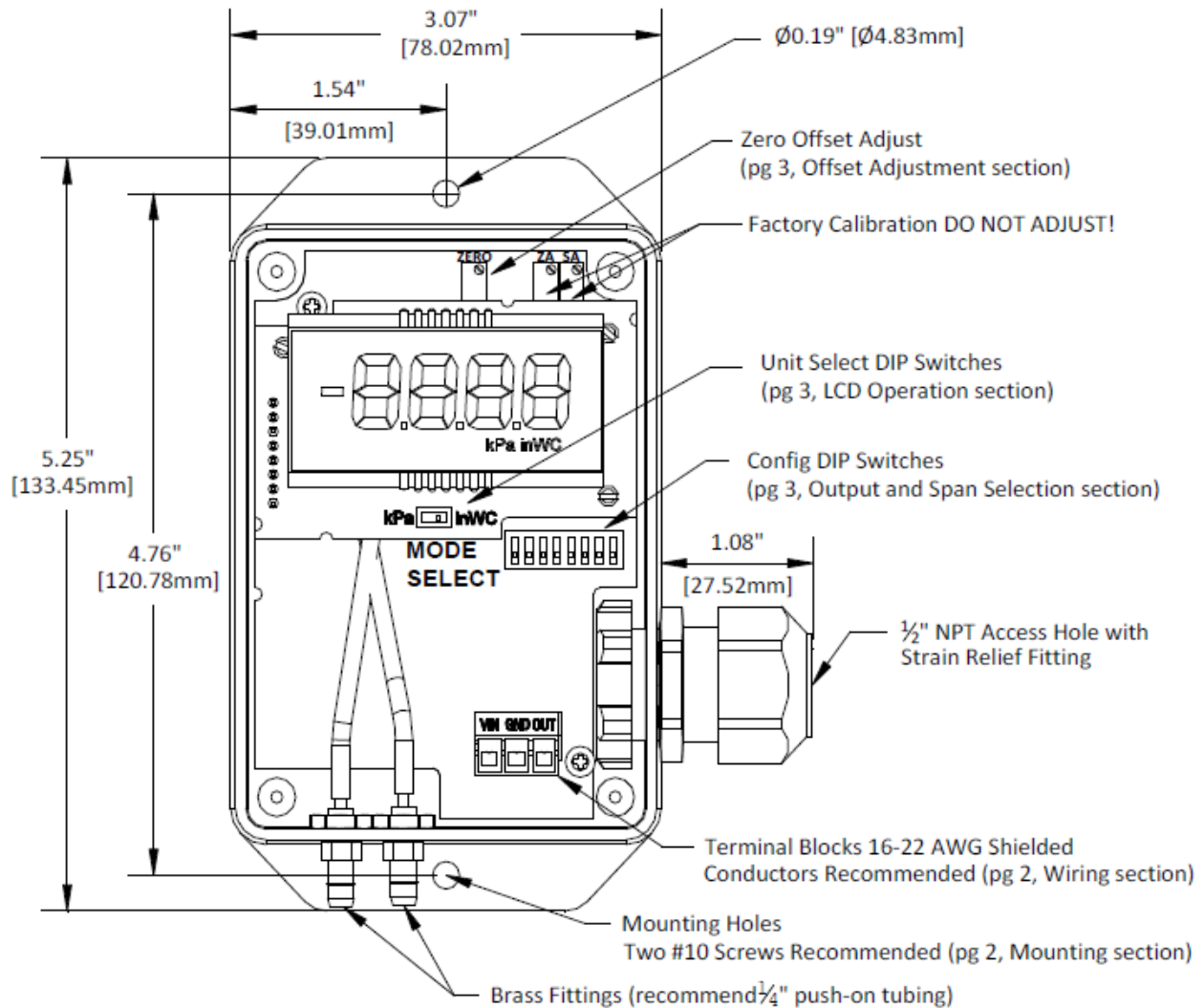
Figure 1: DPA II Differential Pressure Transmitter Dimensions and Hardware
