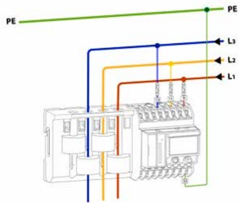
(b) With CT4 Current Module
