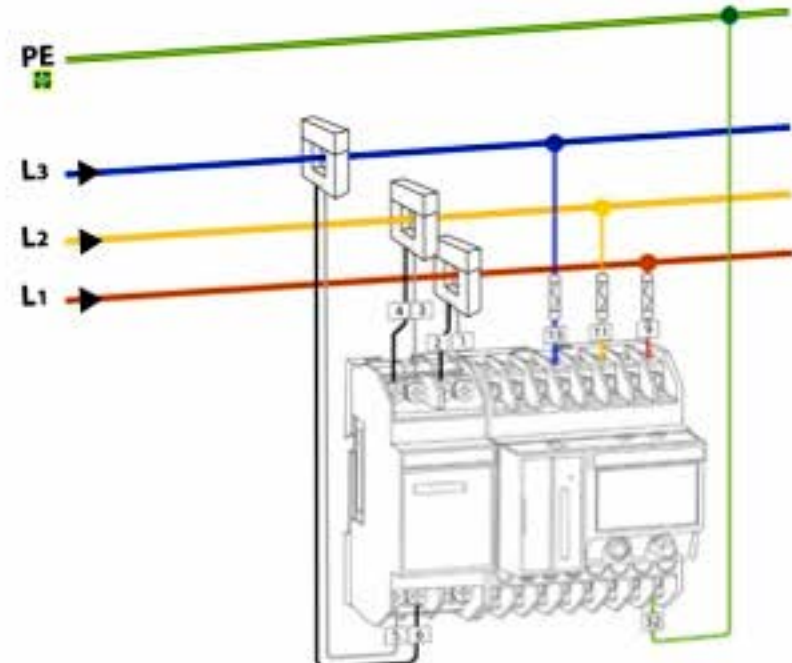
(d) With XCT4 Current Module, 3 current transformers – PQube measures current on all phases
