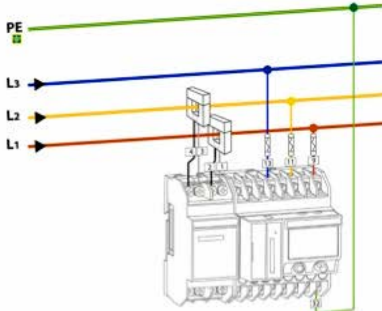
(c) With XCT4 Current Module, 2 current transformers – PQube calculates current on third phase
