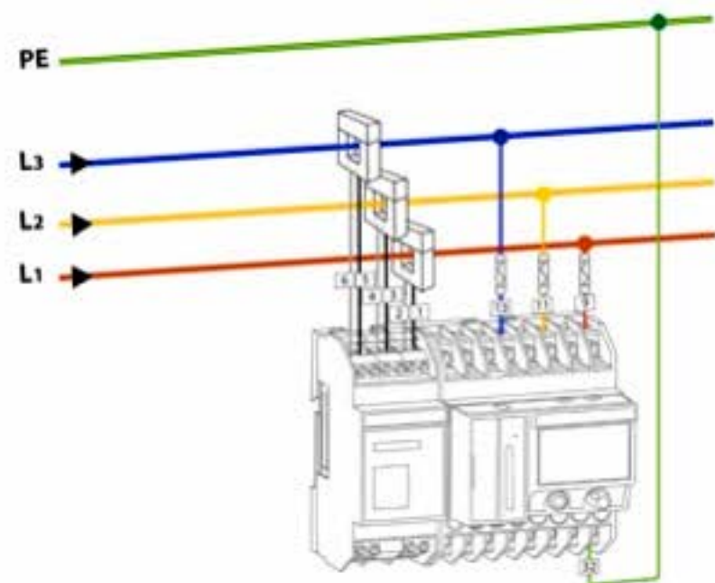
(f) With XCT5/CTE1 Current Module, 3 current transformers – PQube measures current on all phases
