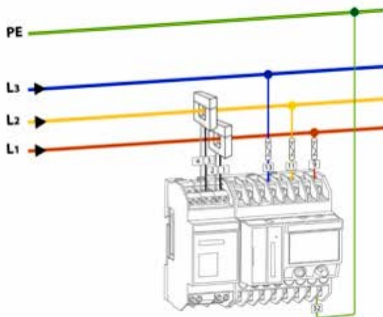
(e) With XCT5/CTE1 Current Module, 2 current transformers – PQube calculates current on third phase
