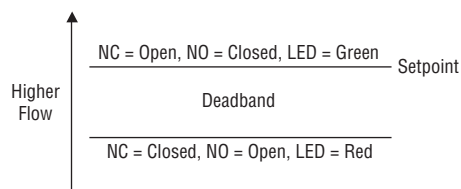
FIGURE 1: Switch Setpoint &amp; Deadband
