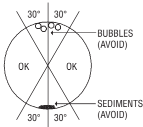
FIGURE 2: Mounting Orientation
