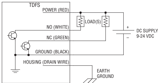
FIGURE 3: Wiring Diagram
