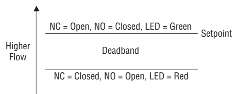
FIGURE 1: Switch Setpoint &amp; Deadband
