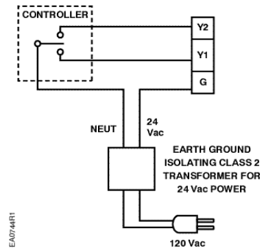
Figure 14. Connecting Terminals (SAV81.00U).
