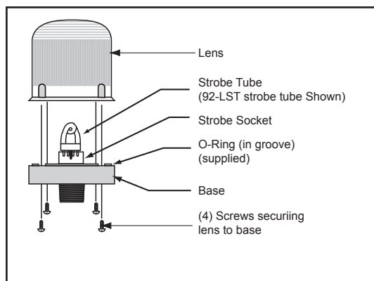
Figure 3. Strobe Tube Replacement
