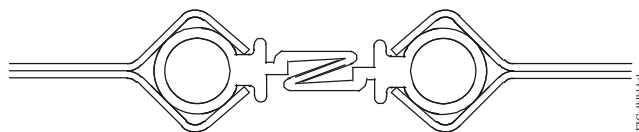
Figure 6: Double-Piece Blade Steel Profile
